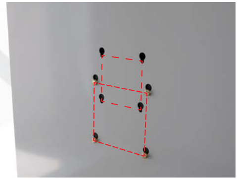
Holes for Vesa 75 or 100 monitor
